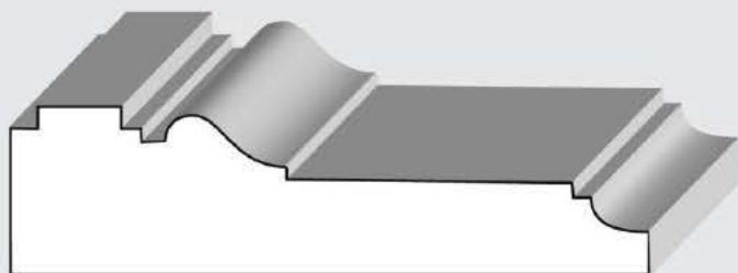
AB654 7/8" x 3-7/16"
